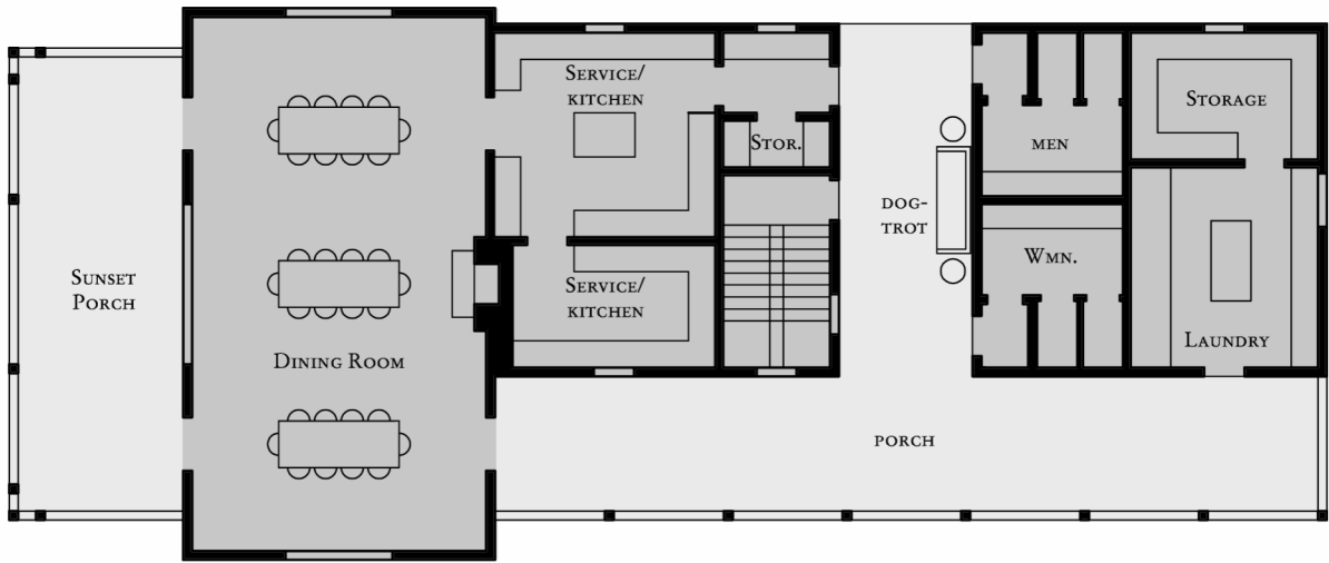
OPTION 1 FIRST FLOOR PLAN
